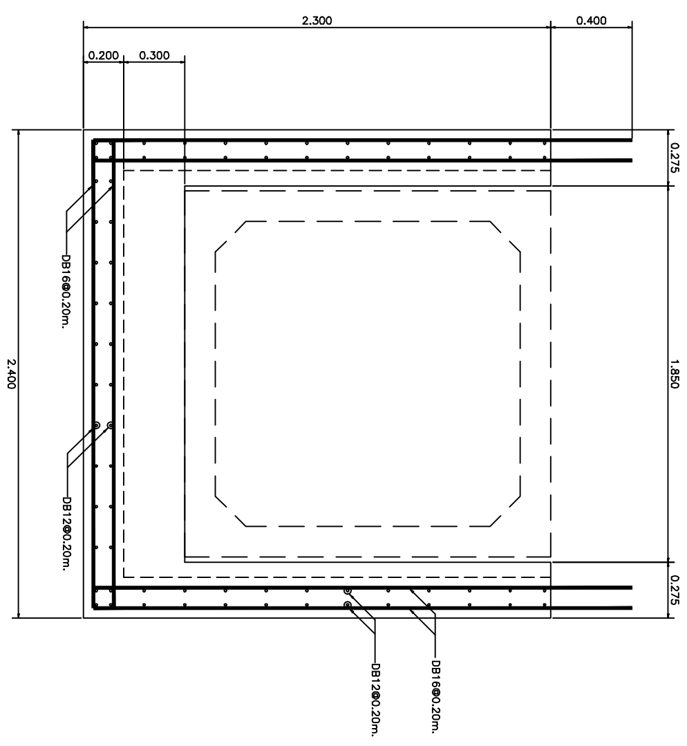
CROSS SECTION
